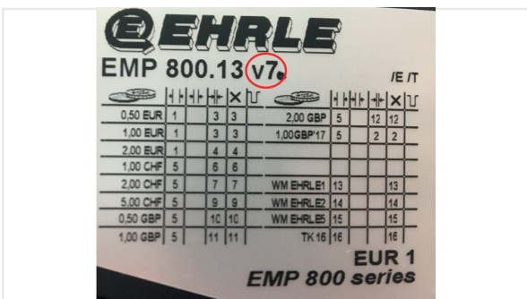
Münzprüfer Version 7 Coin acceptor version 7
